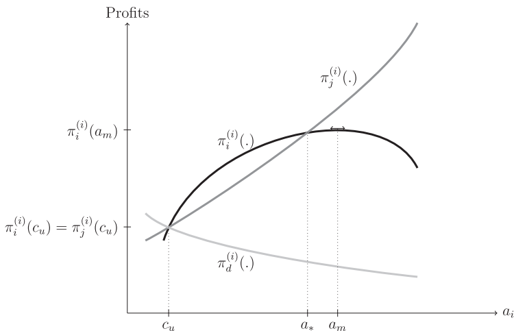
Figure 2 Profits in the Symmetric Linear Case ( \gamma \geq \bar{\gamma} )
